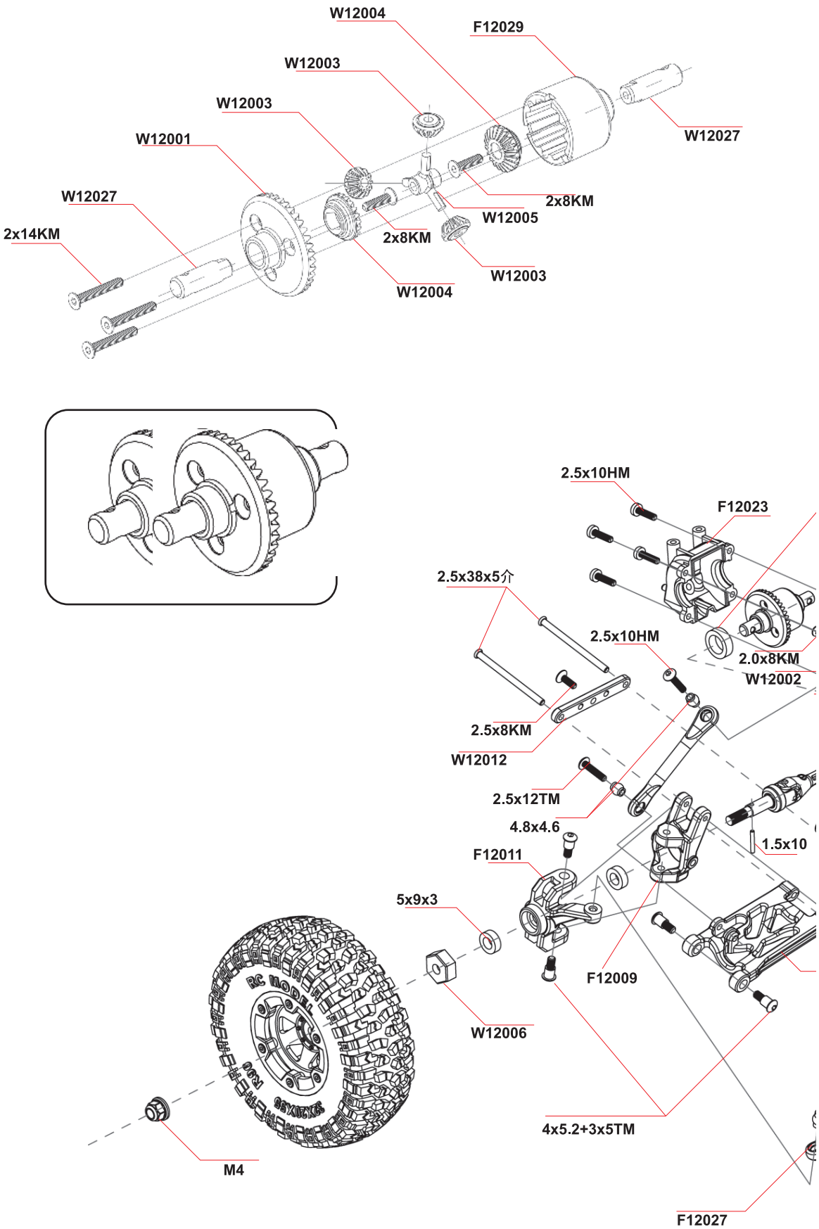
Front gear box exploded view
