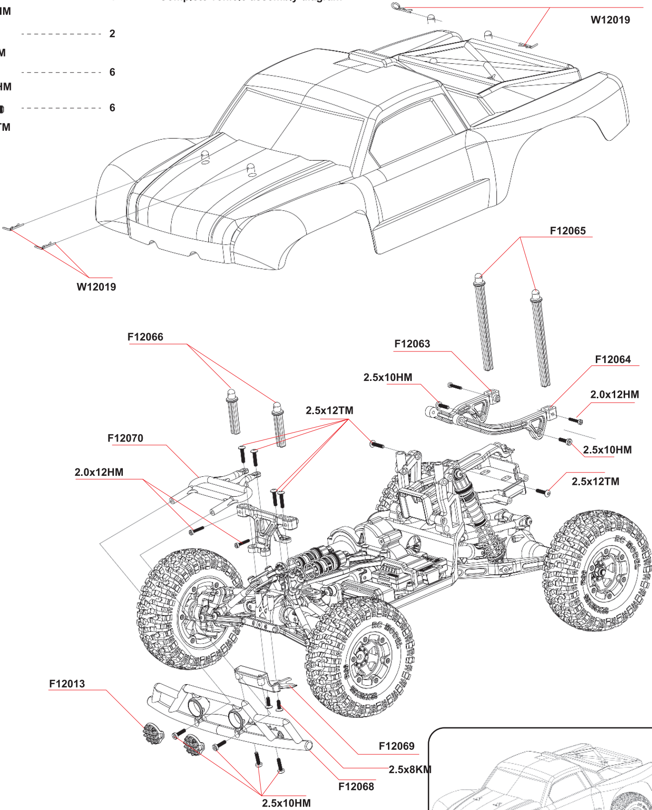
Complete vehicle assembly diagram
