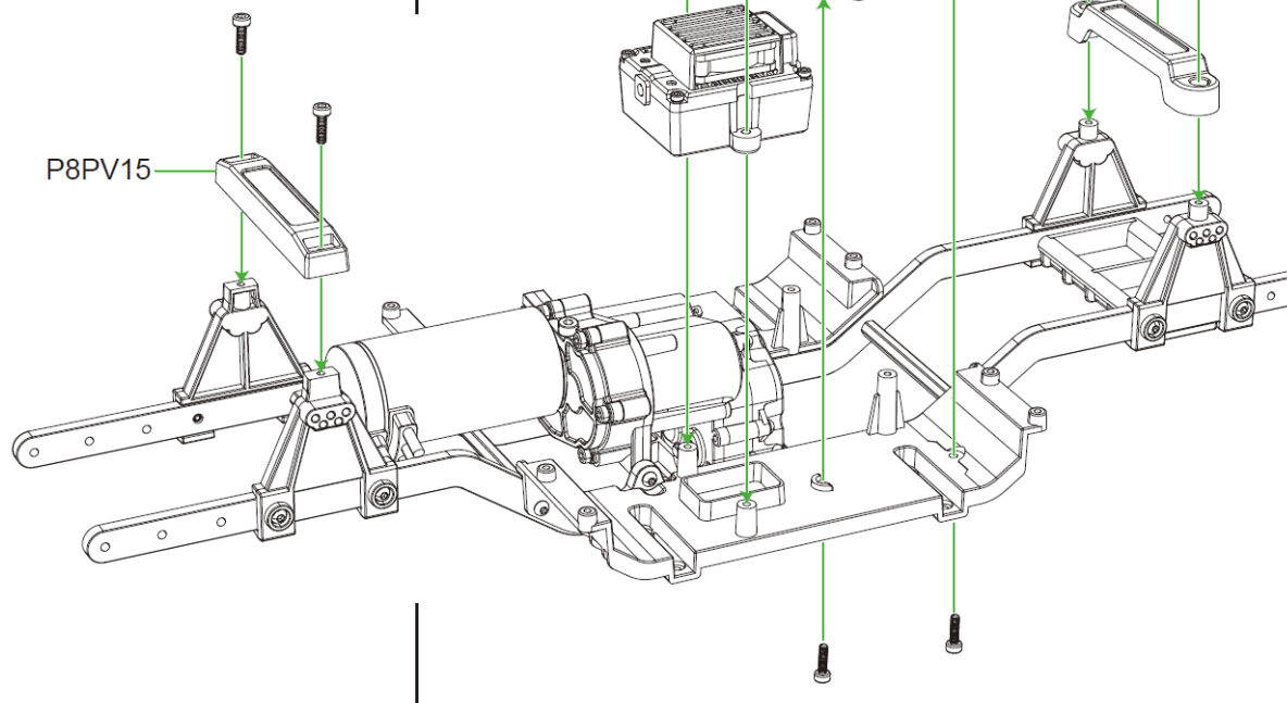
HHM3080 Ø3x8mm Screw Schraube
