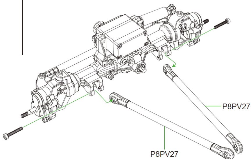
HMM3018 Ø3x18mm Screw Schraube
